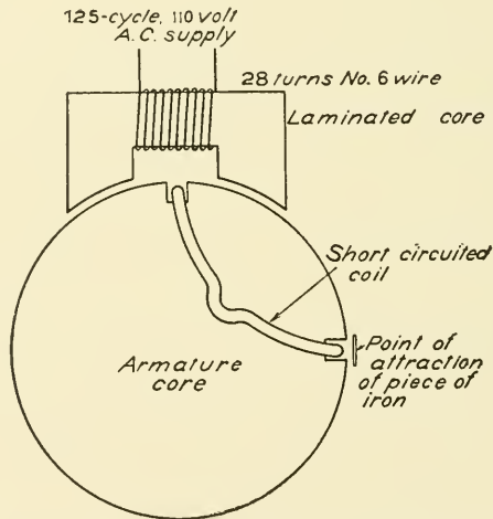
Fig. 135. Diagram Showing "Transformer Test"
